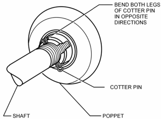
FIGURE 5 – POPPET/COTTER PIN INSTALLATION
